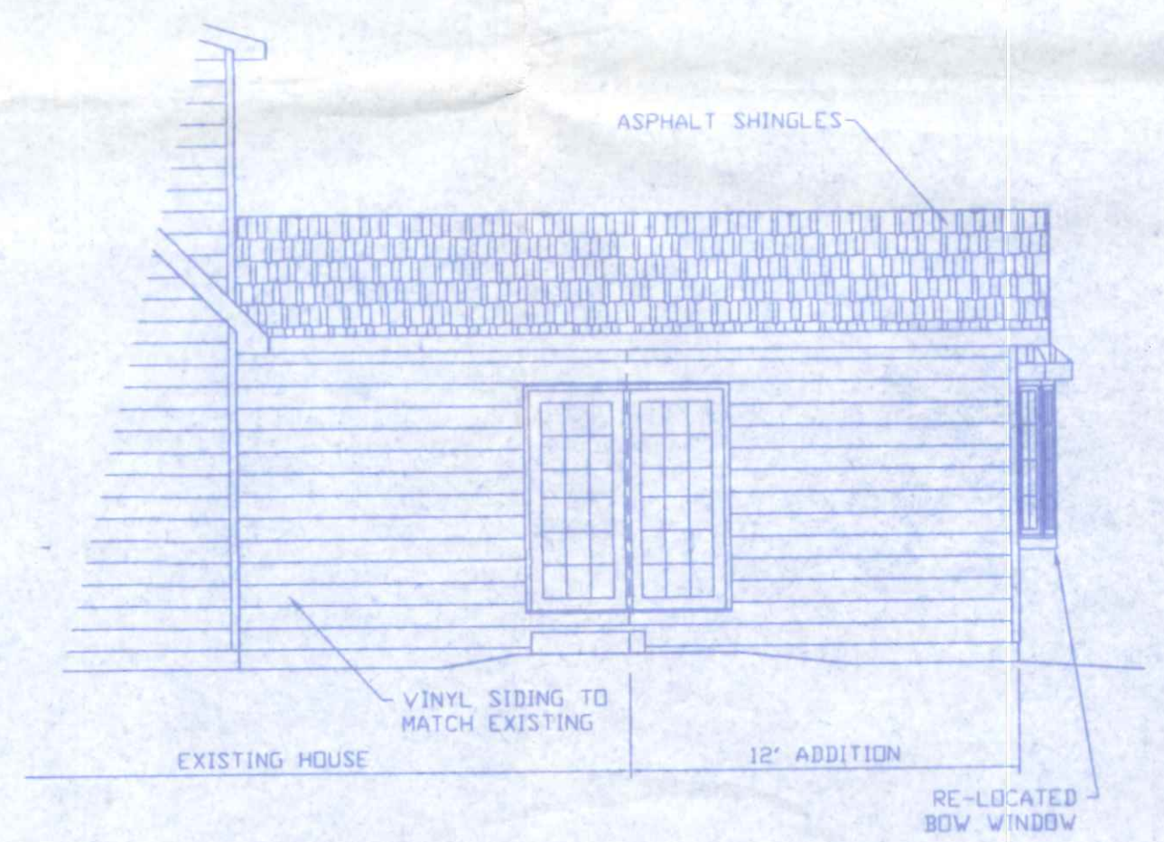
RIGHT SIDE ELEVATION 3/16" = 1'-0"
